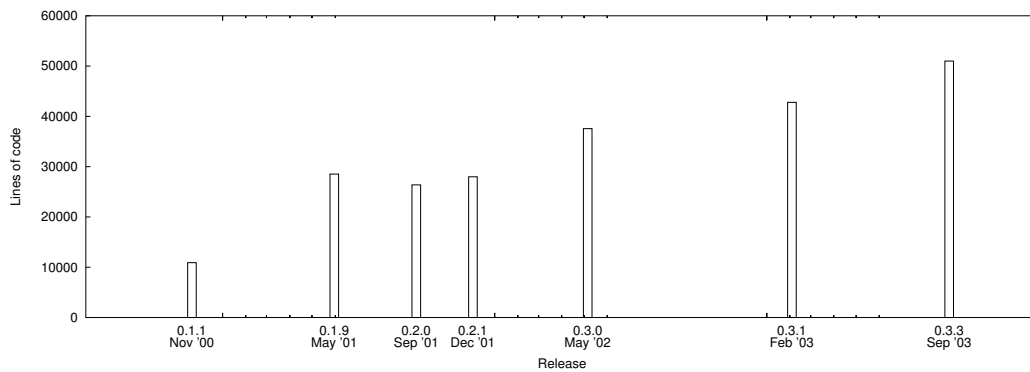
Figure 1: total lines of code as a function of the released version
