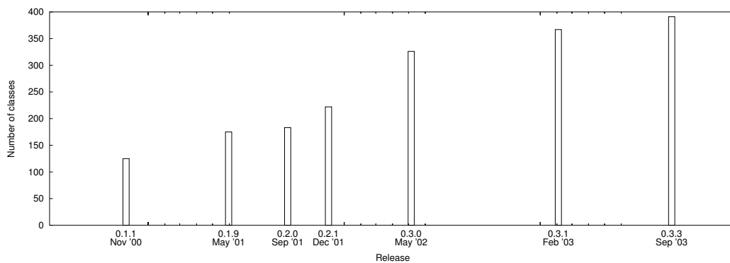
Figure 2: number of public classes as a function of the released version
